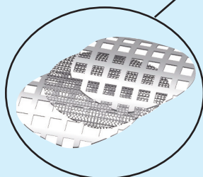
angular filter with strainer "type sandwich"
